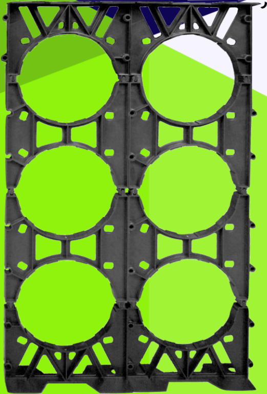
Duct Bank –example of duct bank assembled at job site, ready for concrete
